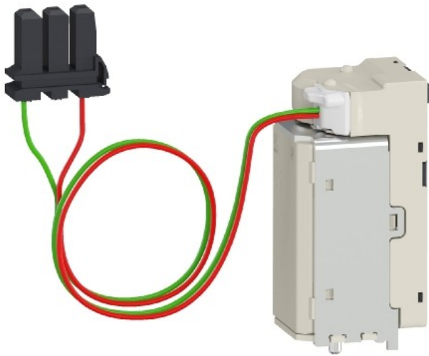
Shunt release
